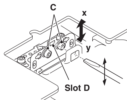
Fig.2-2 Moving of Slot D
