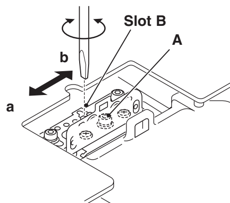
Fig.2-1 Moving of slot B
