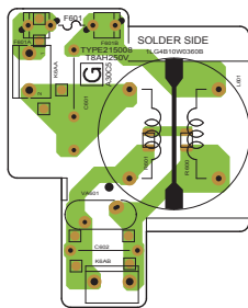
LINE FILTER (SIDE:B)
